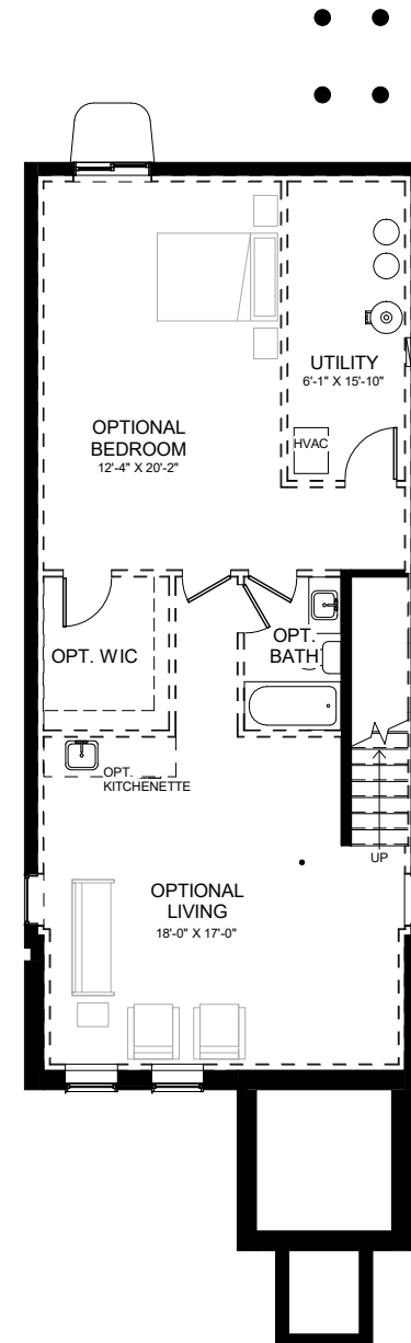
BASEMENT PLAN
