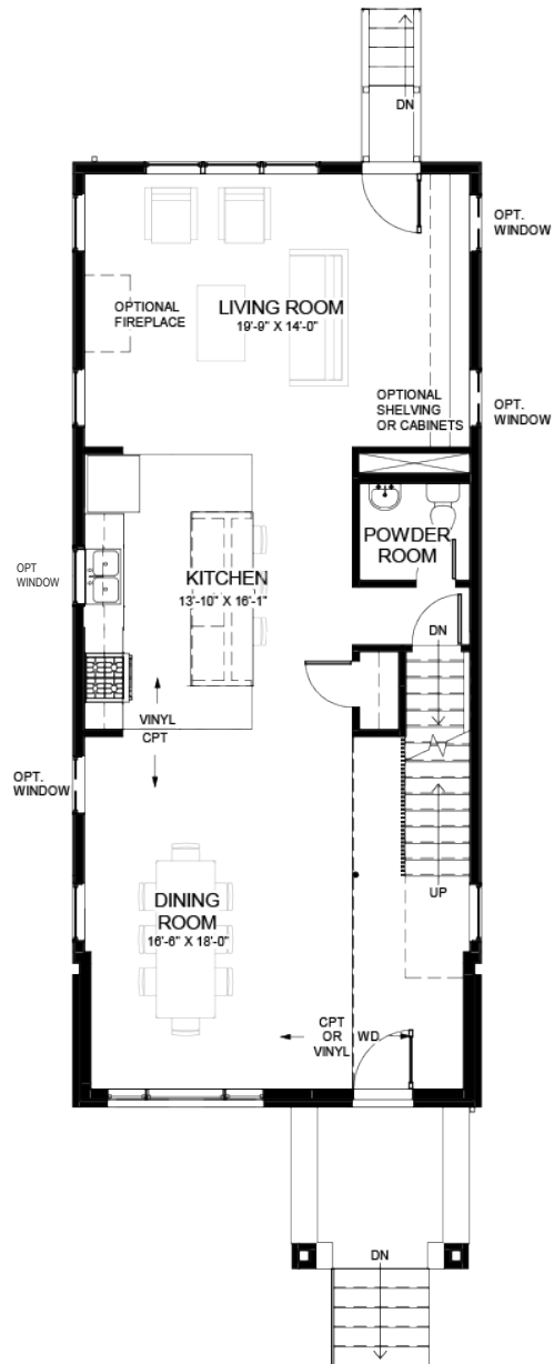
FIRST FLOOR PLAN 1,000 SF
