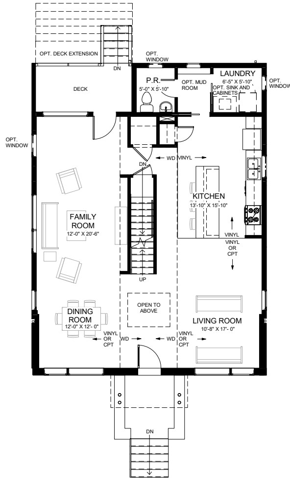
FIRST FLOOR PLAN 1,155 SF
