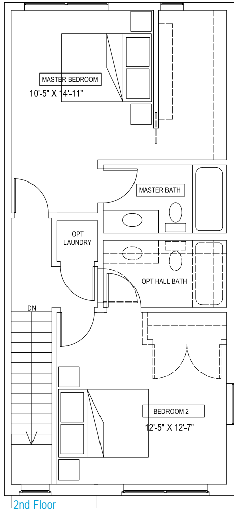
2nd Floor
