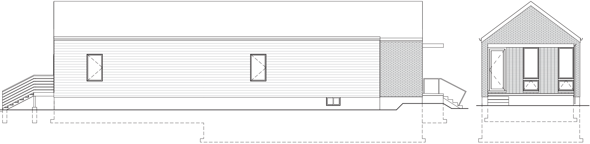
LEFT ELEVATION
